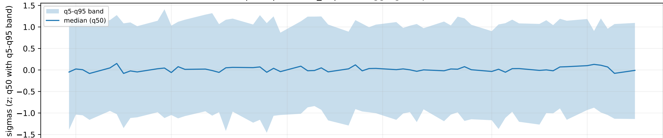
latest | FRA | external_fx | block aggregate quantile bands
